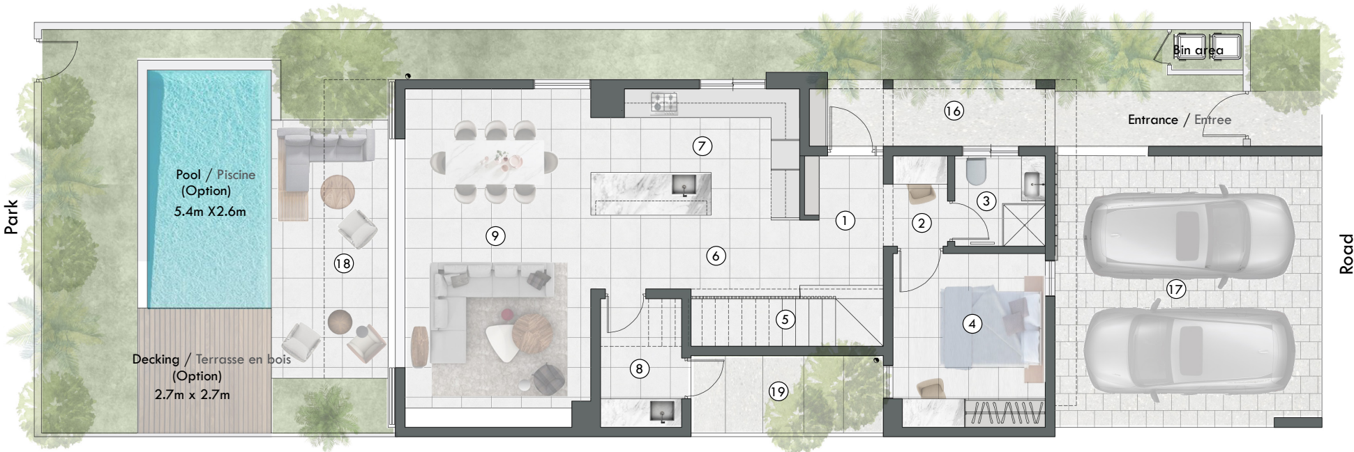
GROUND FLOOR Rez de chausse
